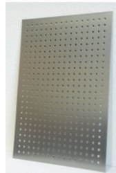
Maßlochung \varnothing 5 mm im Raster 16 x 16 mm Abstand Perforated plate \varnothing 5 mm in the raster 16 x 16 mm distance
