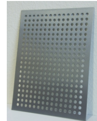
Maßlochung \varnothing 8 mm im Raster 15 x 15 mm Abstand Perforated plate \varnothing 8 mm in the raster 15 x 15 mm distance
